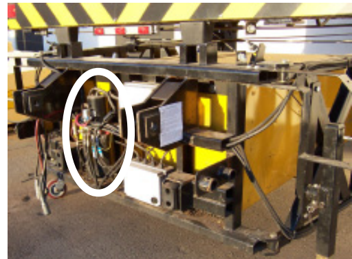
9181 Pump Location
